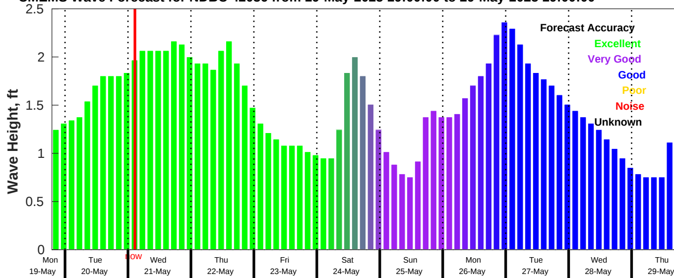
CMEMS Wave Forecast for NDBC 42036 from 19-May-2025 19:00:00 to 29-May-2025 19:00:00
