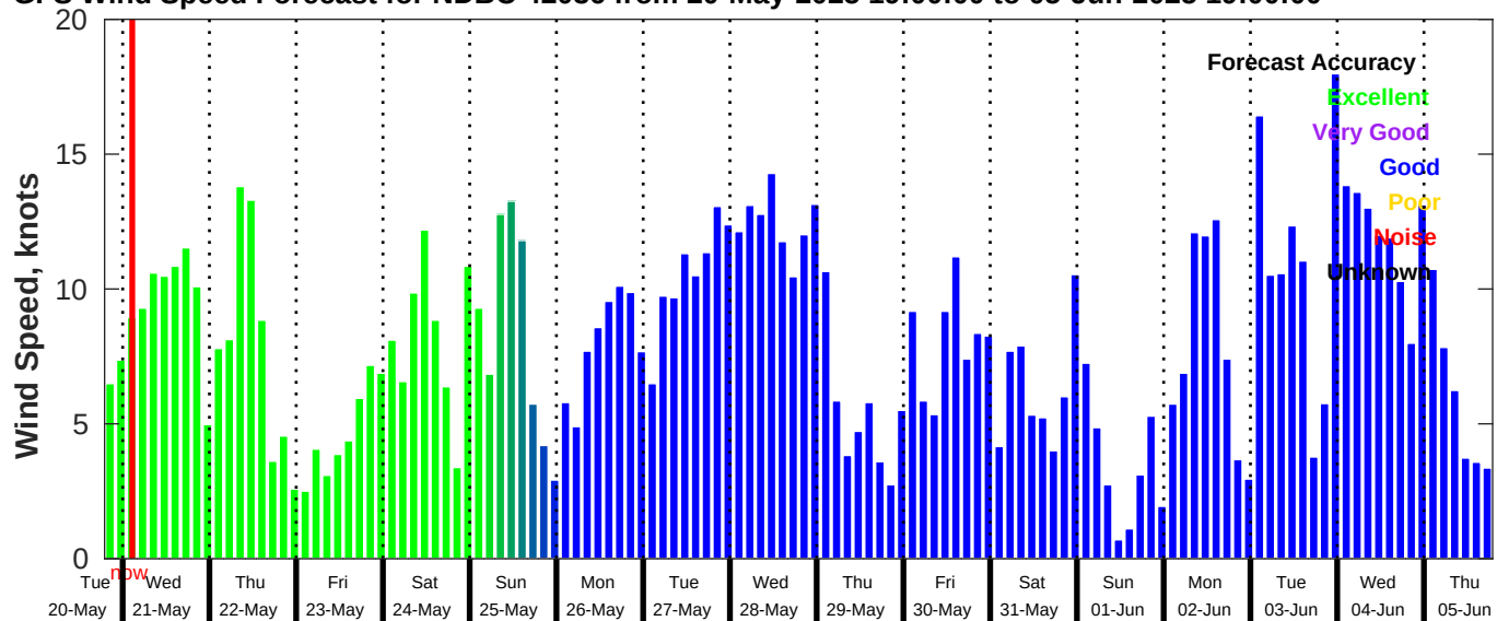
GFS Wind Speed Forecast for NDBC 42036 from 20-May-2025 19:00:00 to 05-Jun-2025 19:00:00
