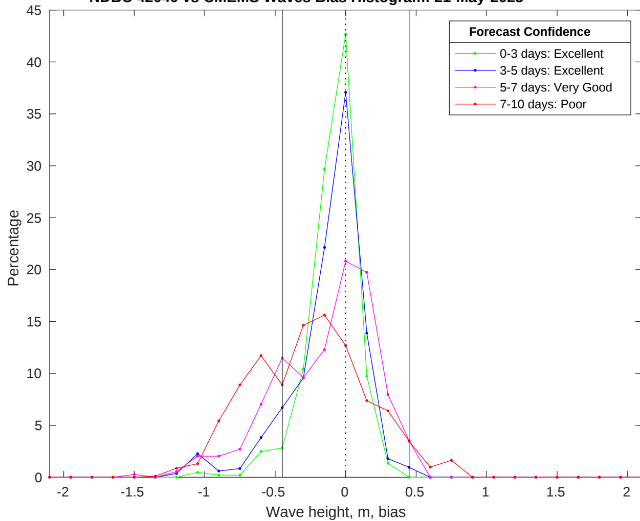
NDBC 42040 vs CMEMS Waves Bias Histogram: 21-May-2025
