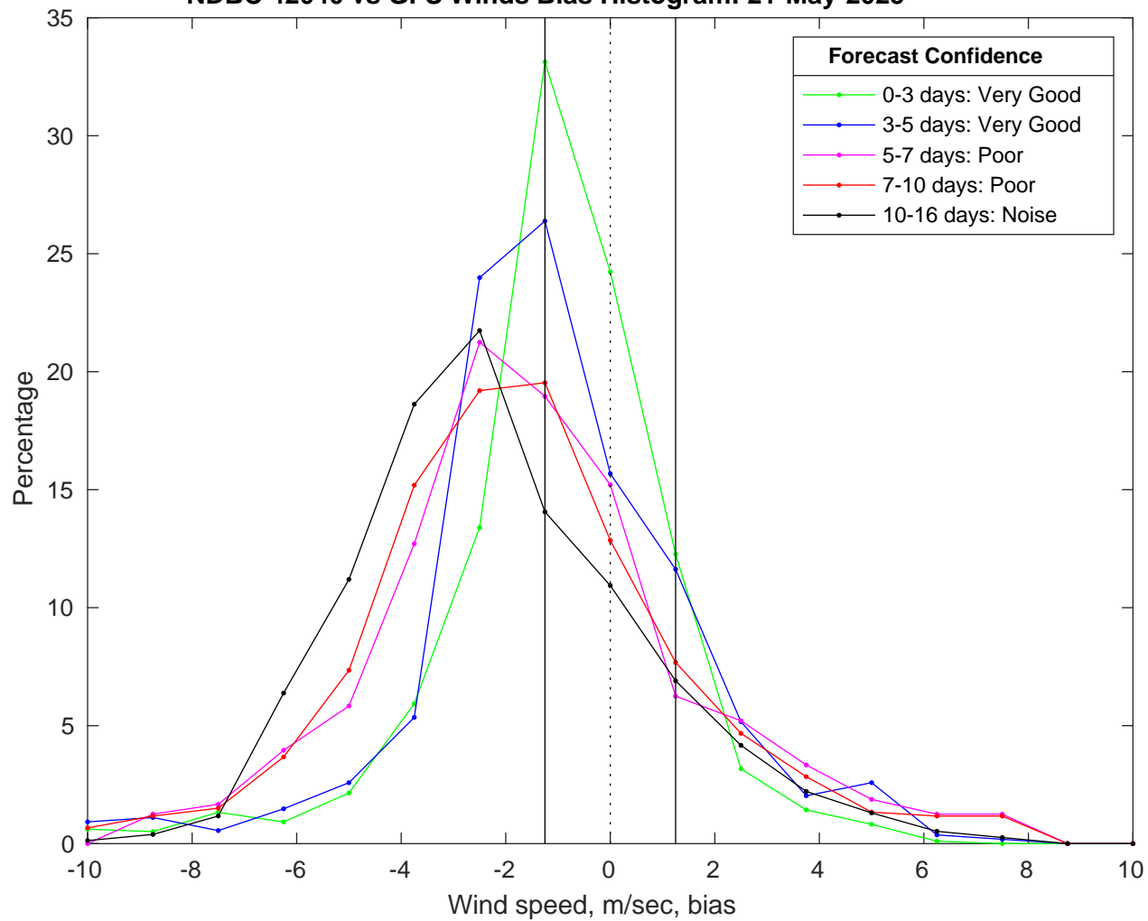
NDBC 42040 vs GFS Winds Bias Histogram: 21-May-2025
