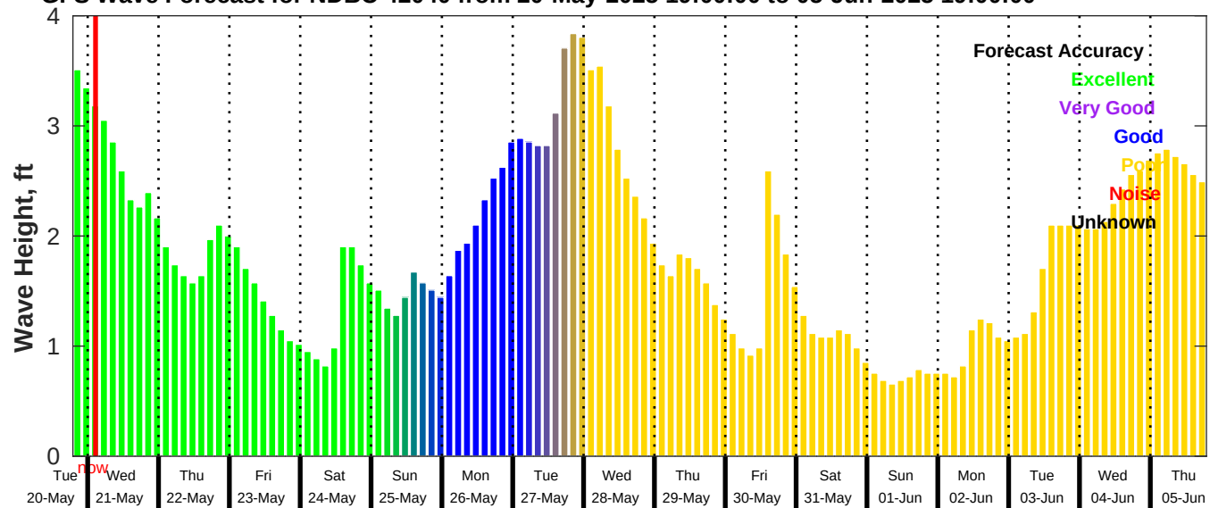
GFS Wave Forecast for NDBC 42040 from 20-May-2025 19:00:00 to 05-Jun-2025 19:00:00
