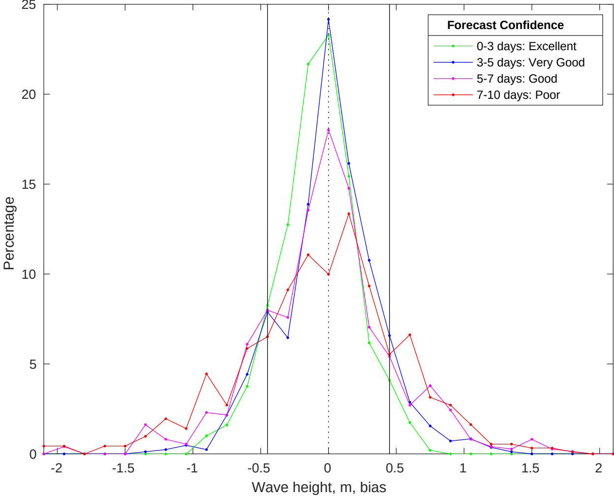
NDBC 46011 vs CMEMS Waves Bias Histogram: 21-May-2025
