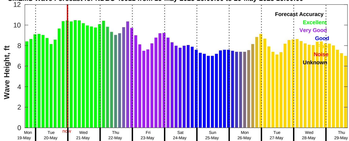
CMEMS Wave Forecast for NDBC 46011 from 19-May-2025 16:00:00 to 29-May-2025 16:00:00
