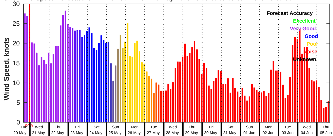
GFS Wind Speed Forecast for NDBC 46011 from 20-May-2025 16:00:00 to 05-Jun-2025 16:00:00
