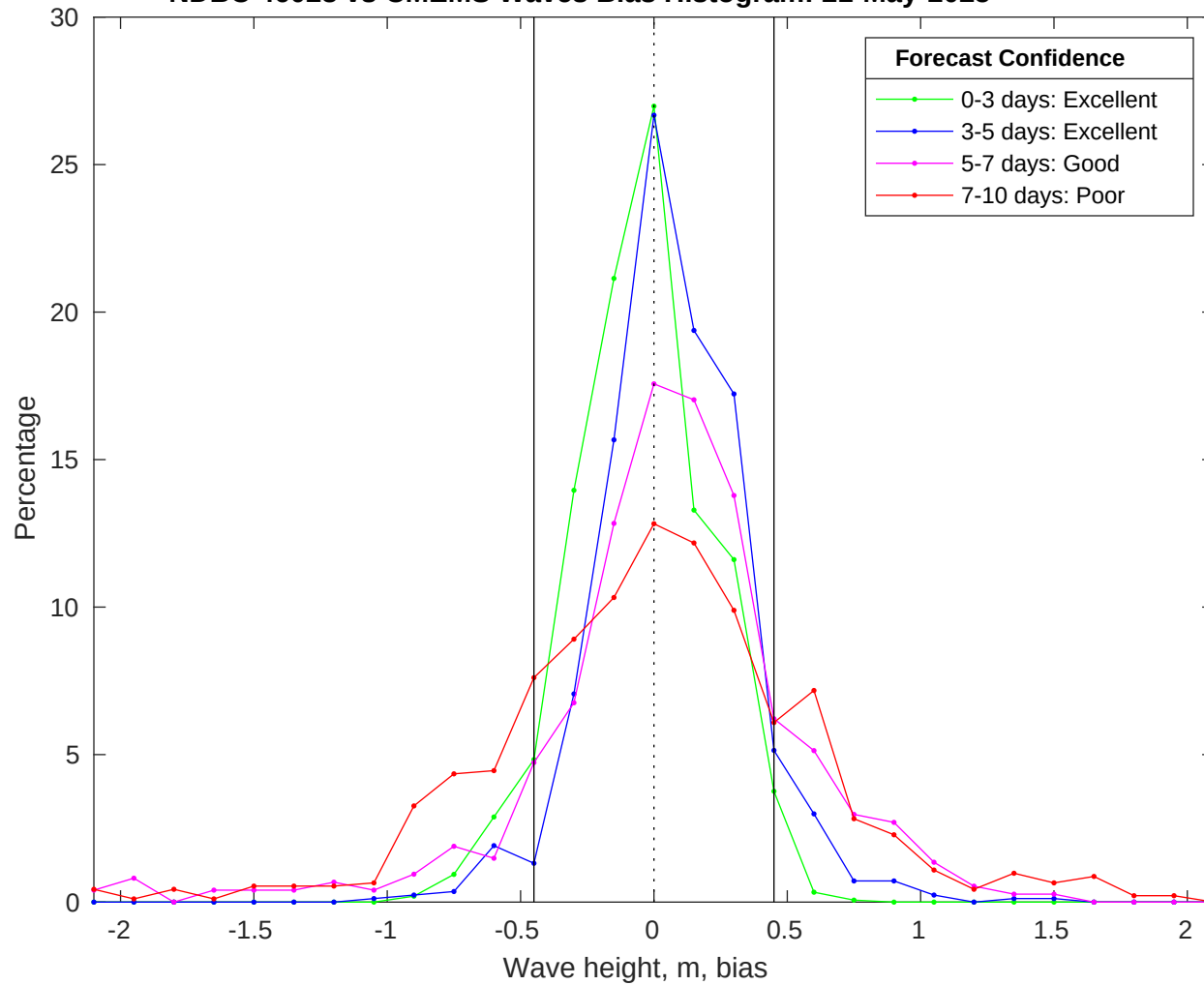
NDBC 46028 vs CMEMS Waves Bias Histogram: 21-May-2025
