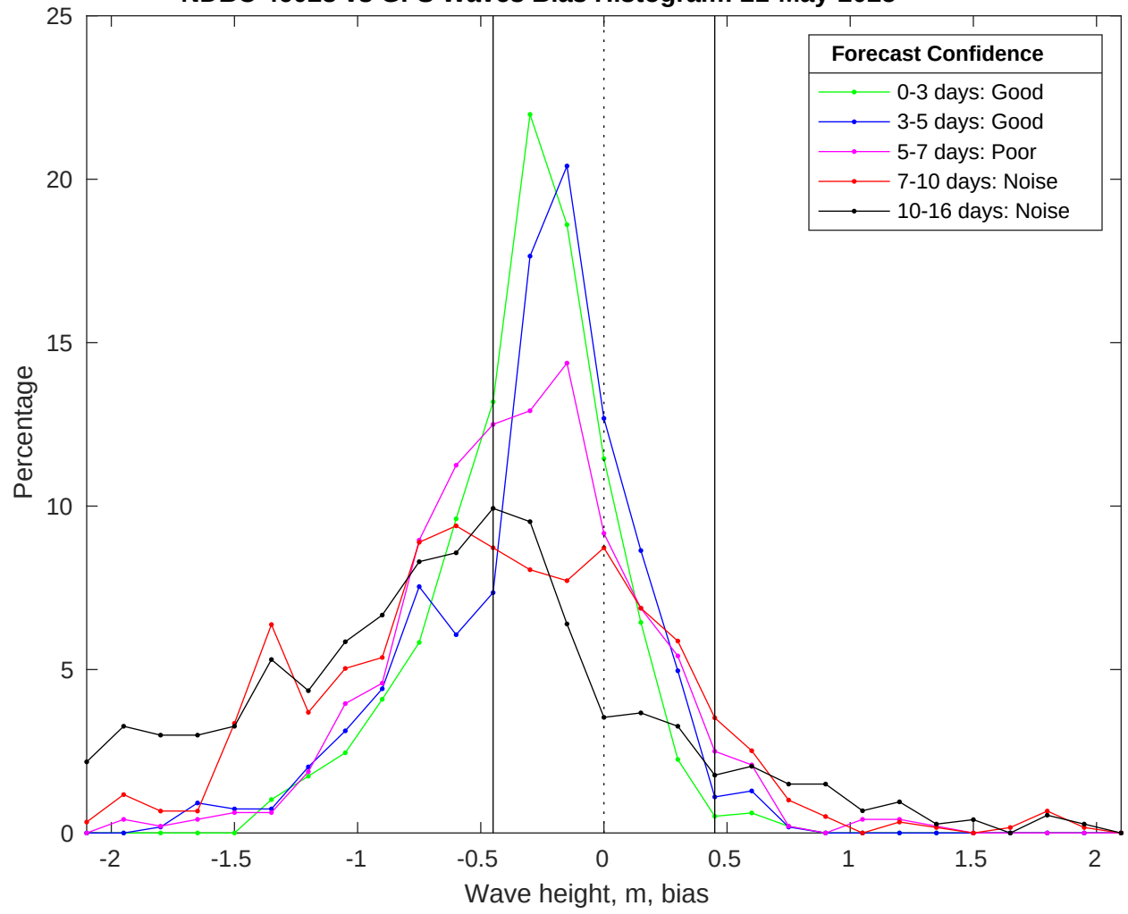
NDBC 46028 vs GFS Waves Bias Histogram: 21-May-2025
