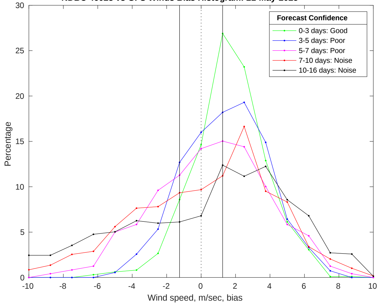
NDBC 46028 vs GFS Winds Bias Histogram: 21-May-2025
