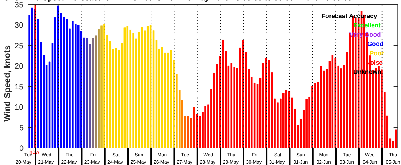
GFS Wind Speed Forecast for NDBC 46028 from 20-May-2025 16:00:00 to 05-Jun-2025 16:00:00
