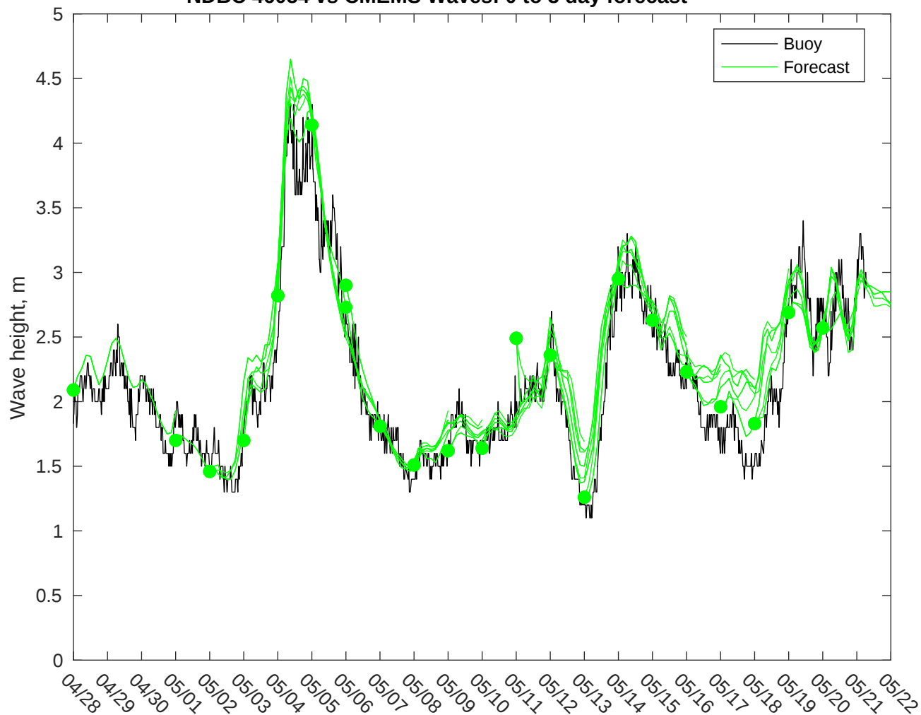
NDBC 46054 vs CMEMS Waves: 0 to 3 day forecast
