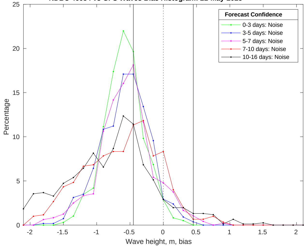
NDBC 46054 vs GFS Waves Bias Histogram: 21-May-2025
