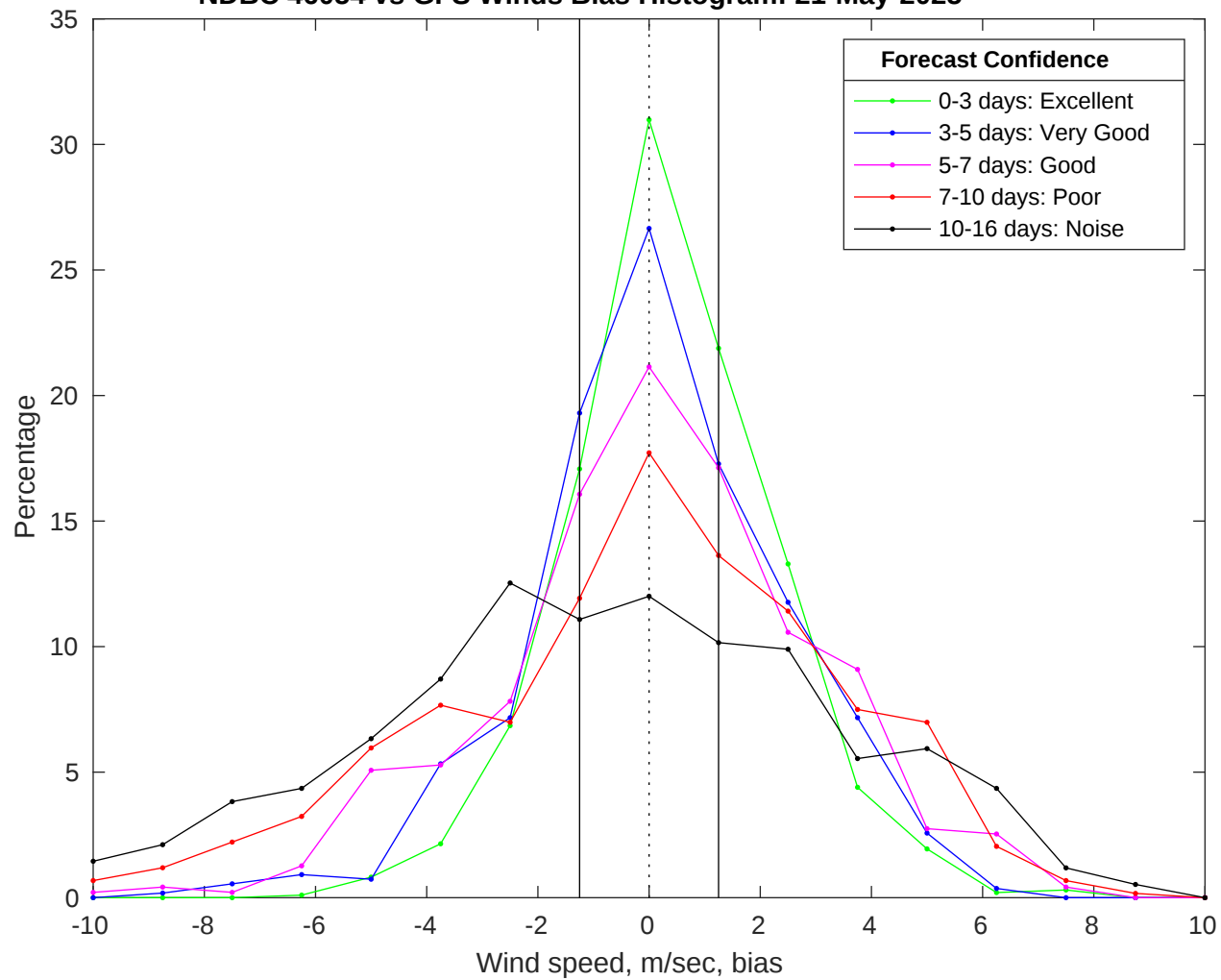
NDBC 46054 vs GFS Winds Bias Histogram: 21-May-2025
