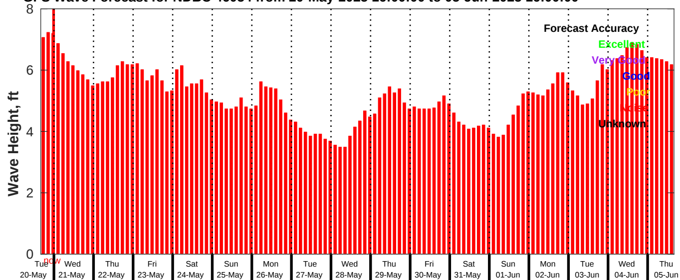
GFS Wave Forecast for NDBC 46054 from 20-May-2025 16:00:00 to 05-Jun-2025 16:00:00
