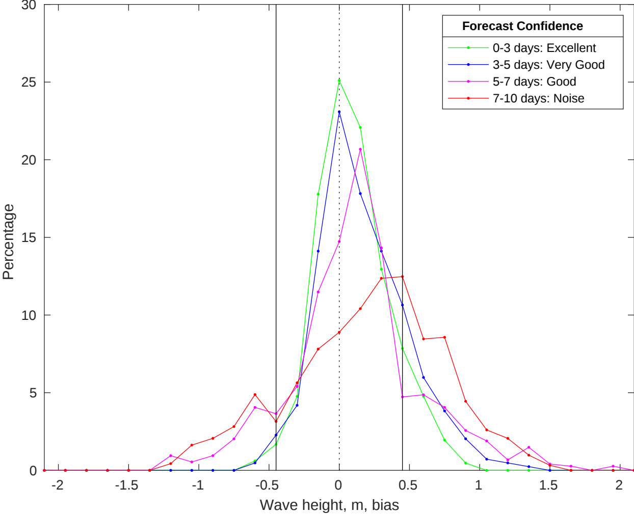
NDBC 46069 vs CMEMS Waves Bias Histogram: 21-May-2025
