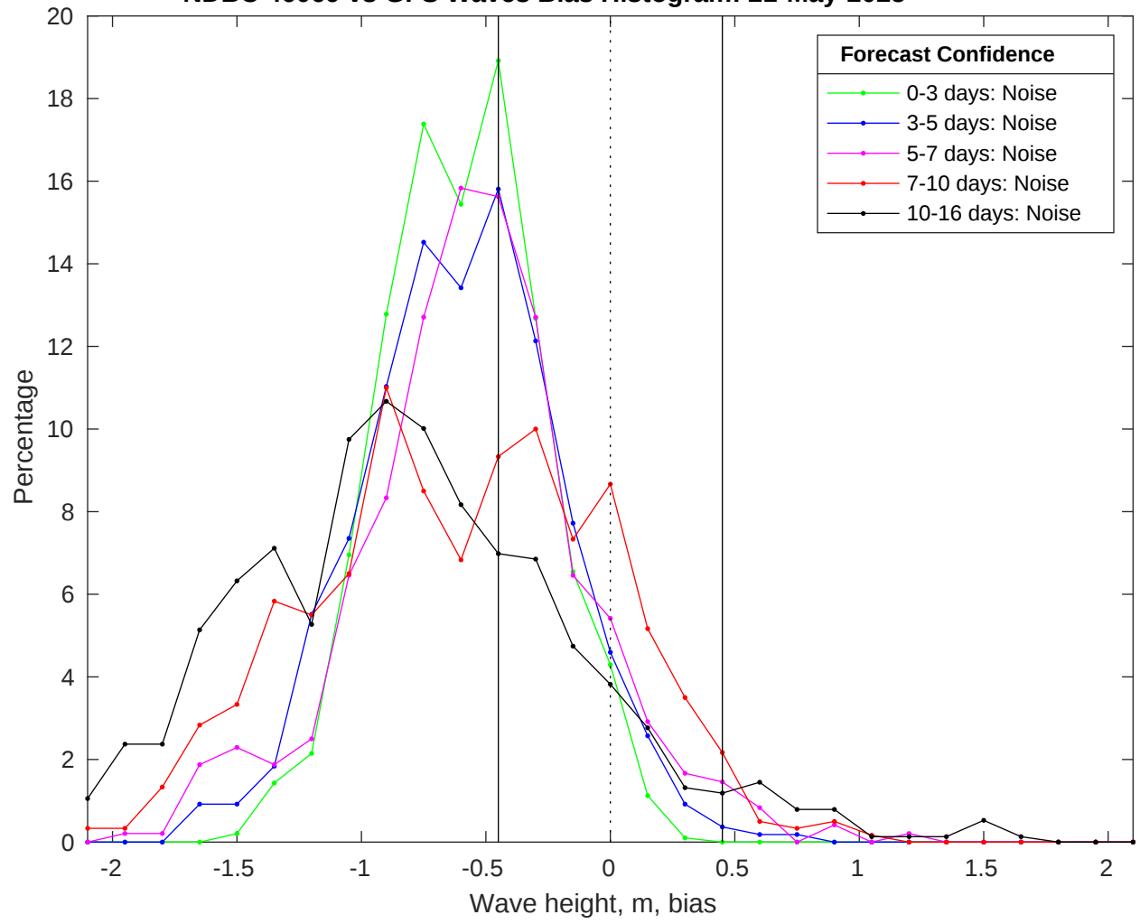
NDBC 46069 vs GFS Waves Bias Histogram: 21-May-2025
