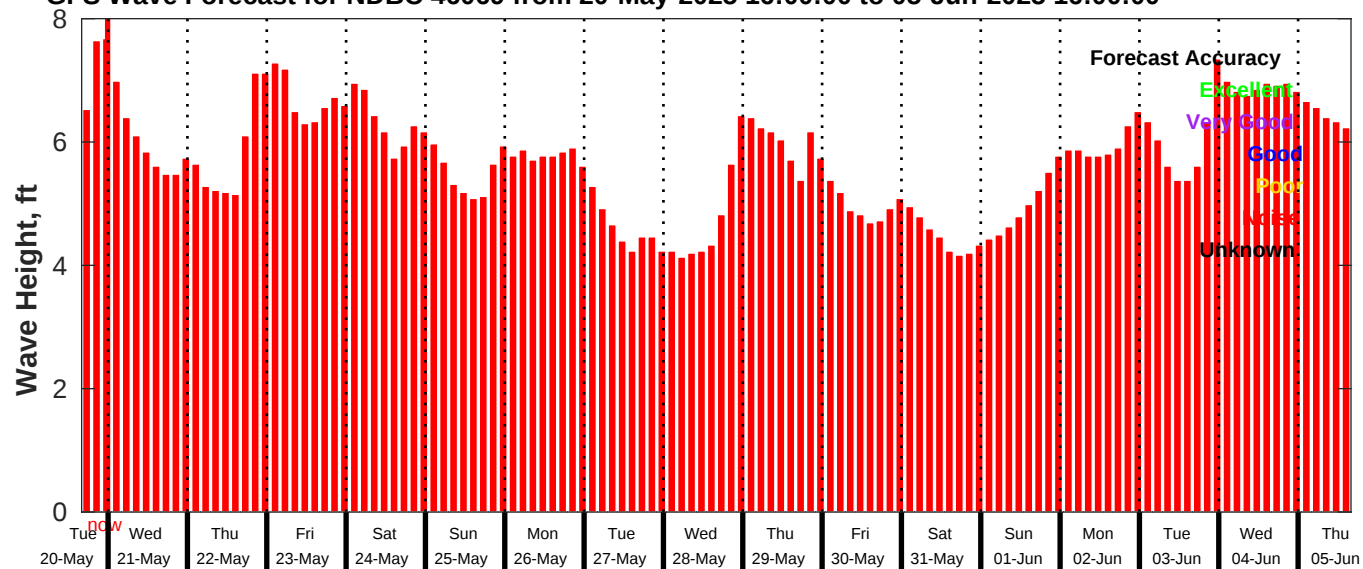
GFS Wave Forecast for NDBC 46069 from 20-May-2025 16:00:00 to 05-Jun-2025 16:00:00
