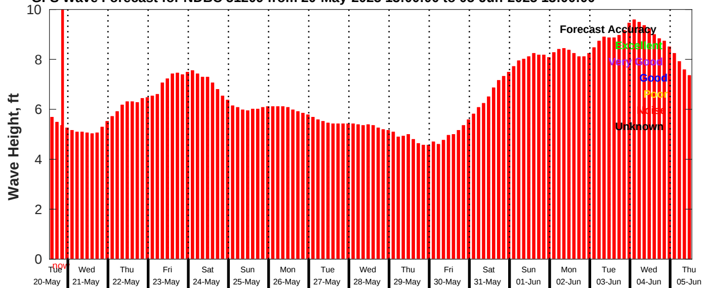
GFS Wave Forecast for NDBC 51209 from 20-May-2025 13:00:00 to 05-Jun-2025 13:00:00
