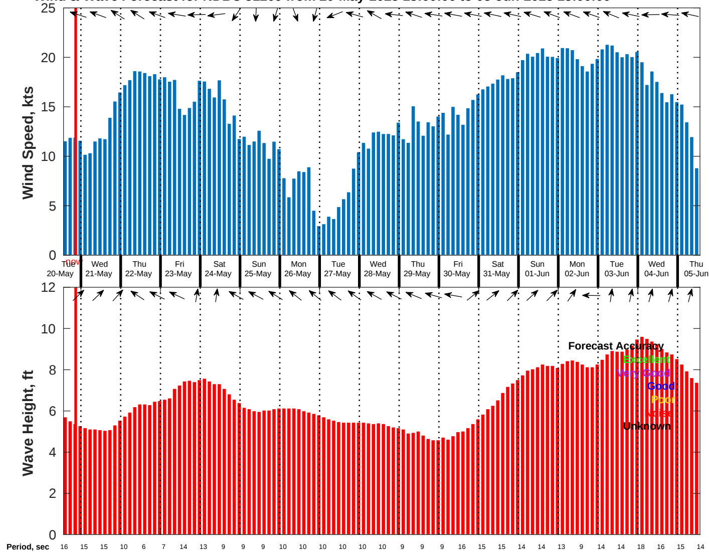
Wind & Wave Forecast for NDBC 51209 from 20-May-2025 13:00:00 to 05-Jun-2025 13:00:00
