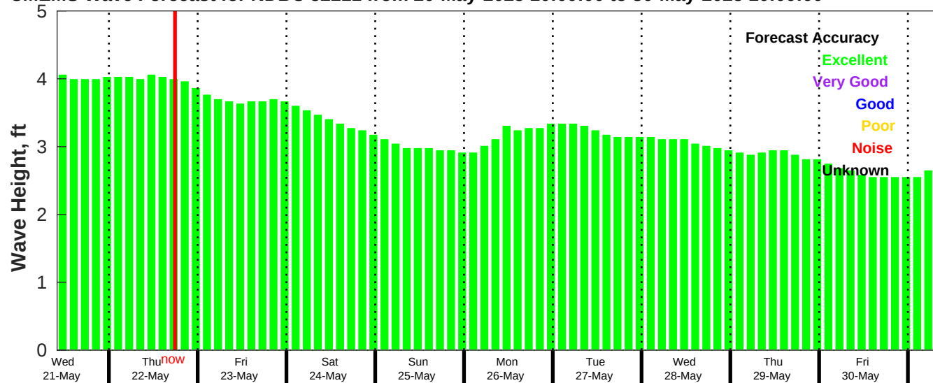
CMEMS Wave Forecast for NDBC 52211 from 20-May-2025 10:00:00 to 30-May-2025 10:00:00
