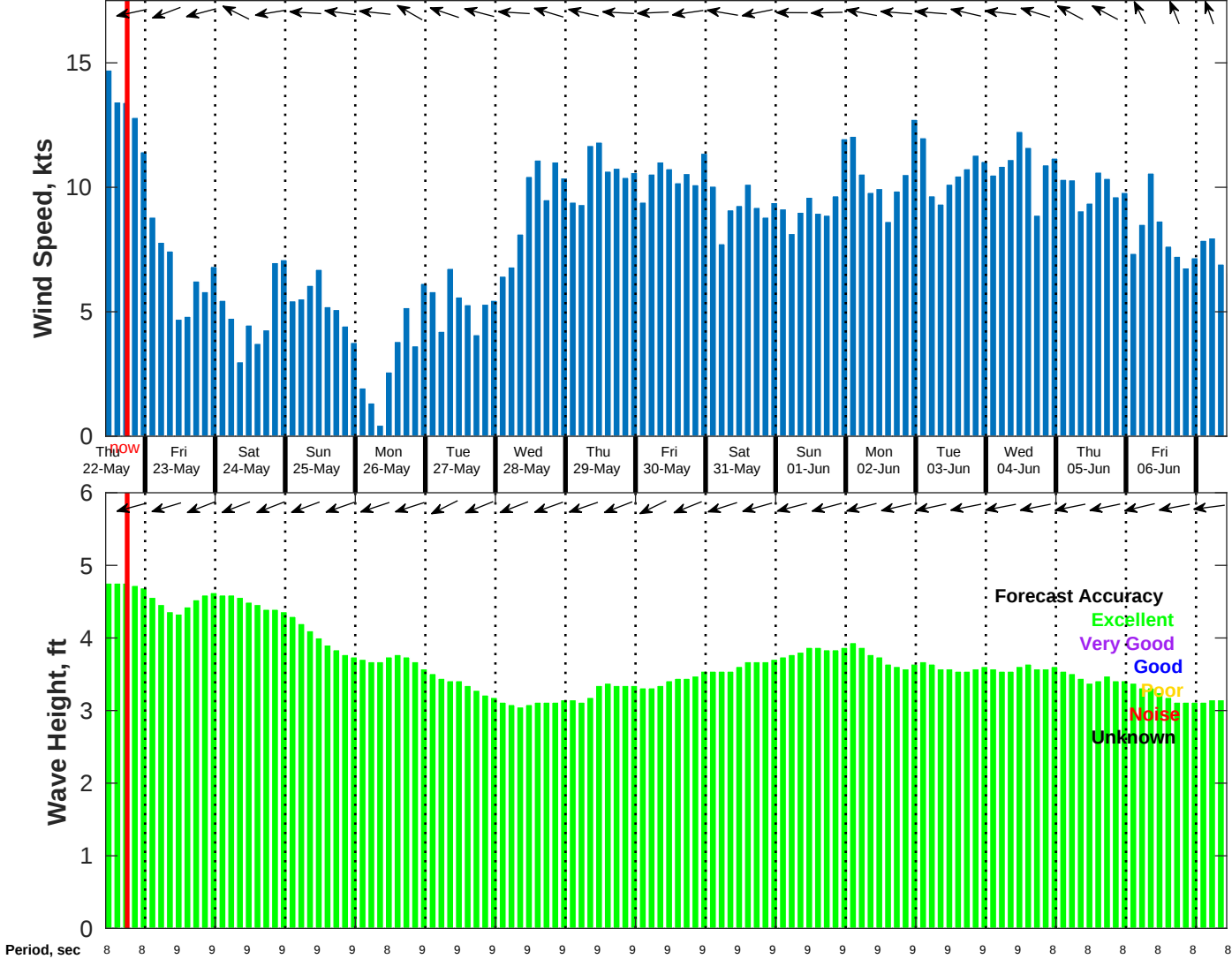
Wind & Wave Forecast for NDBC 52211 from 21-May-2025 10:00:00 to 06-Jun-2025 10:00:00
