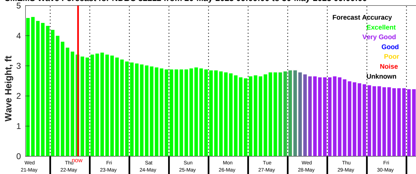
CMEMS Wave Forecast for NDBC 52212 from 20-May-2025 09:00:00 to 30-May-2025 09:00:00
