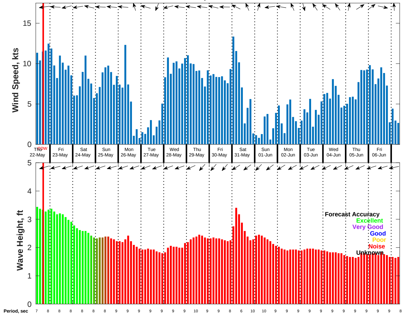
Wind & Wave Forecast for NDBC 52212 from 21-May-2025 09:00:00 to 06-Jun-2025 09:00:00
