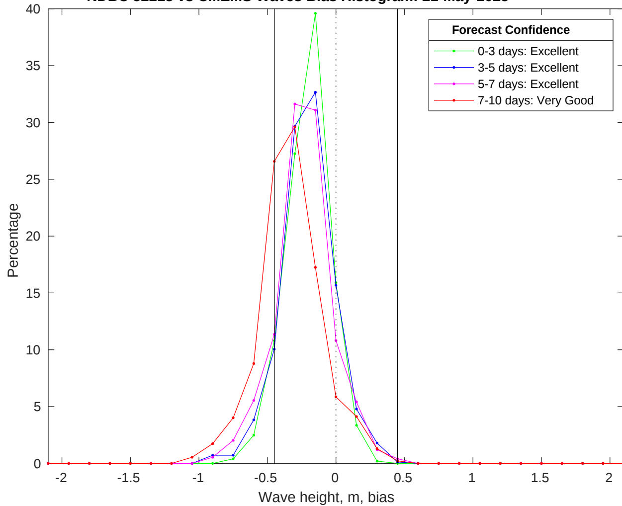
NDBC 52213 vs CMEMS Waves Bias Histogram: 21-May-2025
