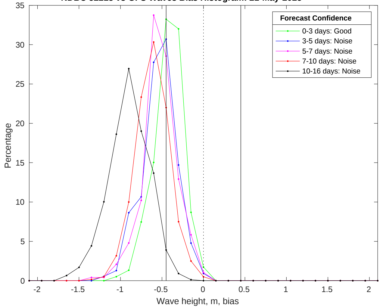
NDBC 52213 vs GFS Waves Bias Histogram: 21-May-2025
