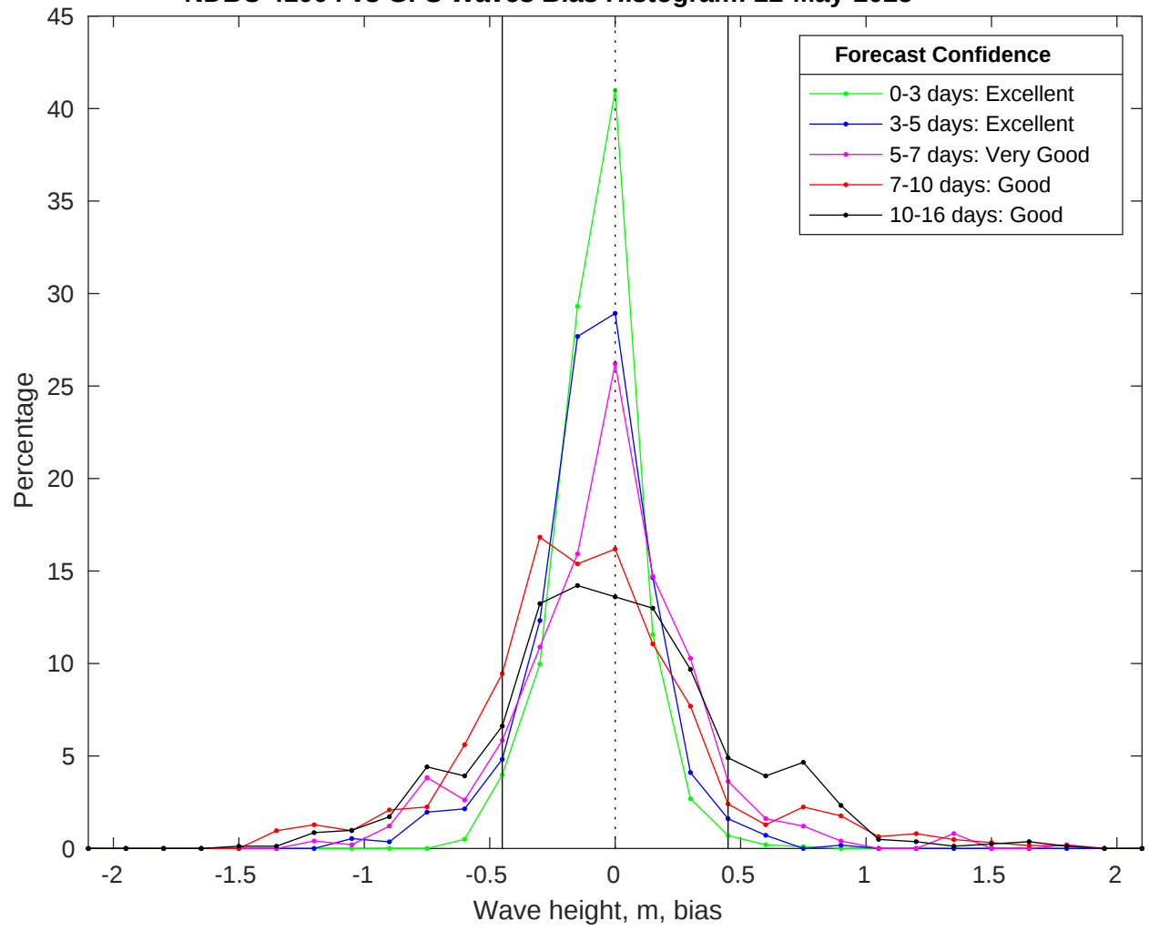
NDBC 41004 vs GFS Waves Bias Histogram: 22-May-2025
