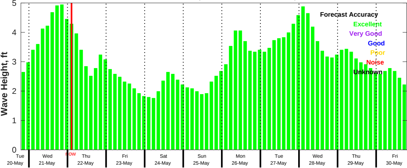
CMEMS Wave Forecast for NDBC 41004 from 20-May-2025 19:00:00 to 30-May-2025 19:00:00
