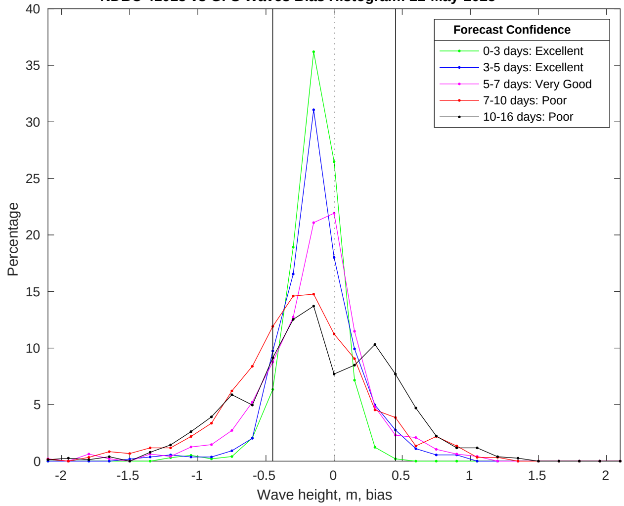
NDBC 41013 vs GFS Waves Bias Histogram: 22-May-2025
