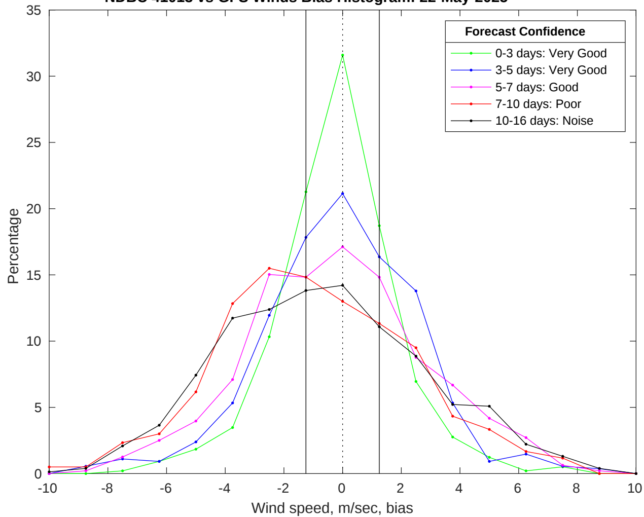
NDBC 41013 vs GFS Winds Bias Histogram: 22-May-2025
