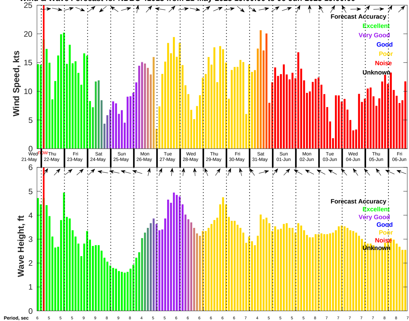
Wind & Wave Forecast for NDBC 41013 from 21-May-2025 19:00:00 to 06-Jun-2025 19:00:00
