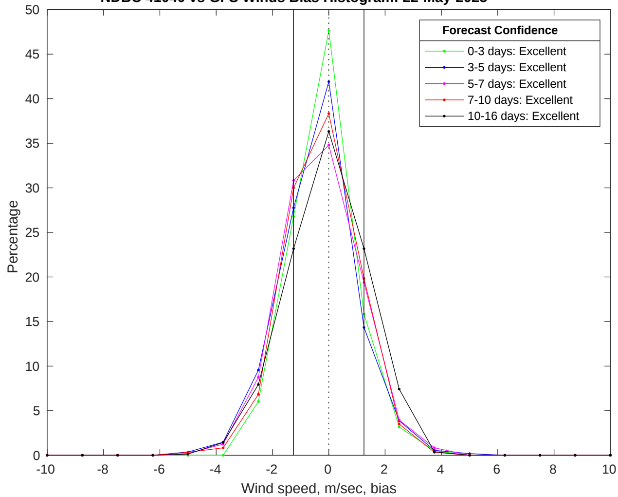
NDBC 41040 vs GFS Winds Bias Histogram: 22-May-2025
