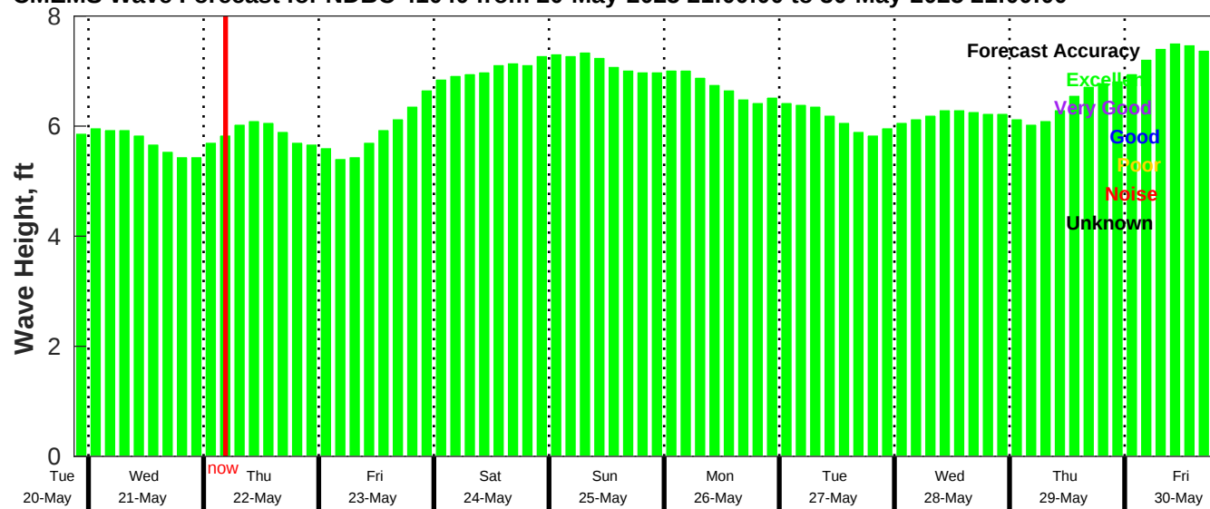
CMEMS Wave Forecast for NDBC 41040 from 20-May-2025 21:00:00 to 30-May-2025 21:00:00
