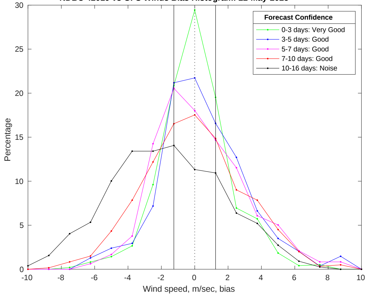
NDBC 42019 vs GFS Winds Bias Histogram: 22-May-2025
