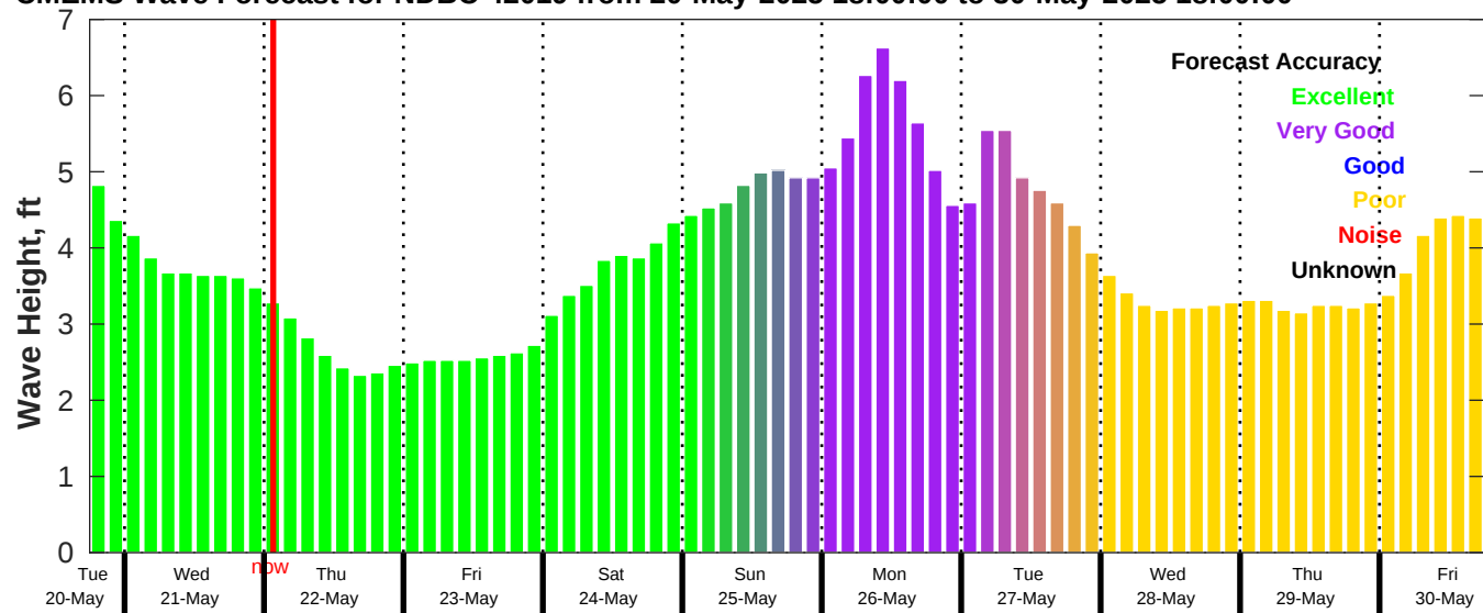
CMEMS Wave Forecast for NDBC 42019 from 20-May-2025 18:00:00 to 30-May-2025 18:00:00
