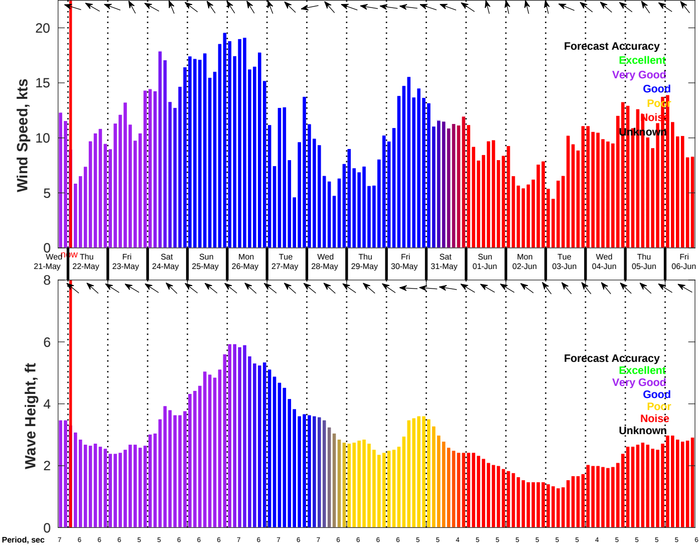
Wind & Wave Forecast for NDBC 42019 from 21-May-2025 18:00:00 to 06-Jun-2025 18:00:00
