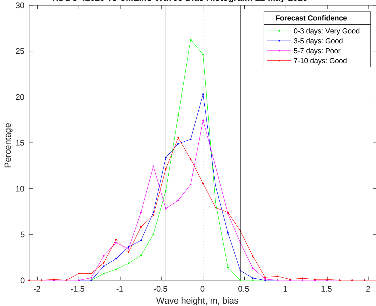
NDBC 42020 vs CMEMS Waves Bias Histogram: 22-May-2025
