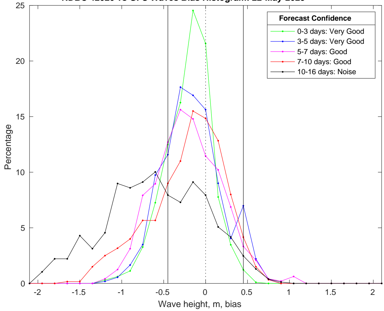
NDBC 42020 vs GFS Waves Bias Histogram: 22-May-2025
