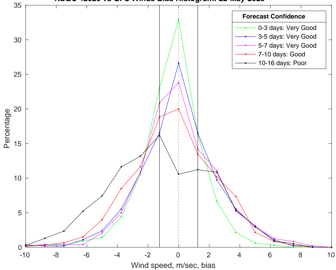
NDBC 42020 vs GFS Winds Bias Histogram: 22-May-2025
