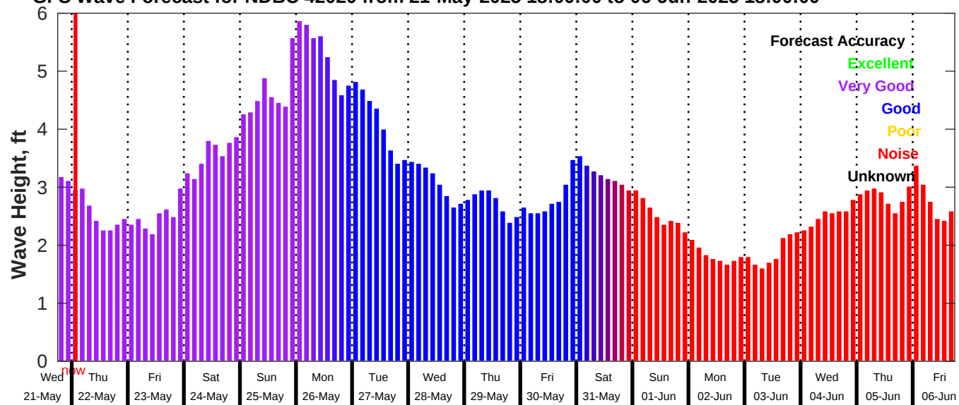
GFS Wave Forecast for NDBC 42020 from 21-May-2025 18:00:00 to 06-Jun-2025 18:00:00
