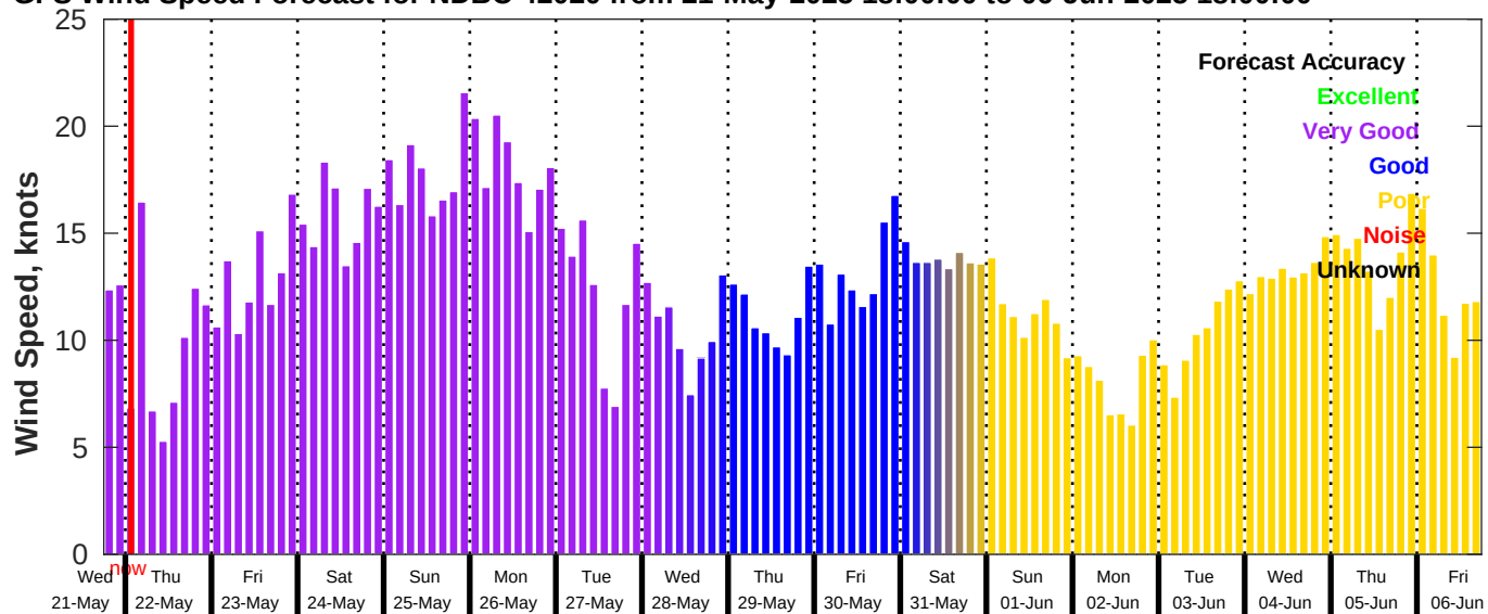
GFS Wind Speed Forecast for NDBC 42020 from 21-May-2025 18:00:00 to 06-Jun-2025 18:00:00
