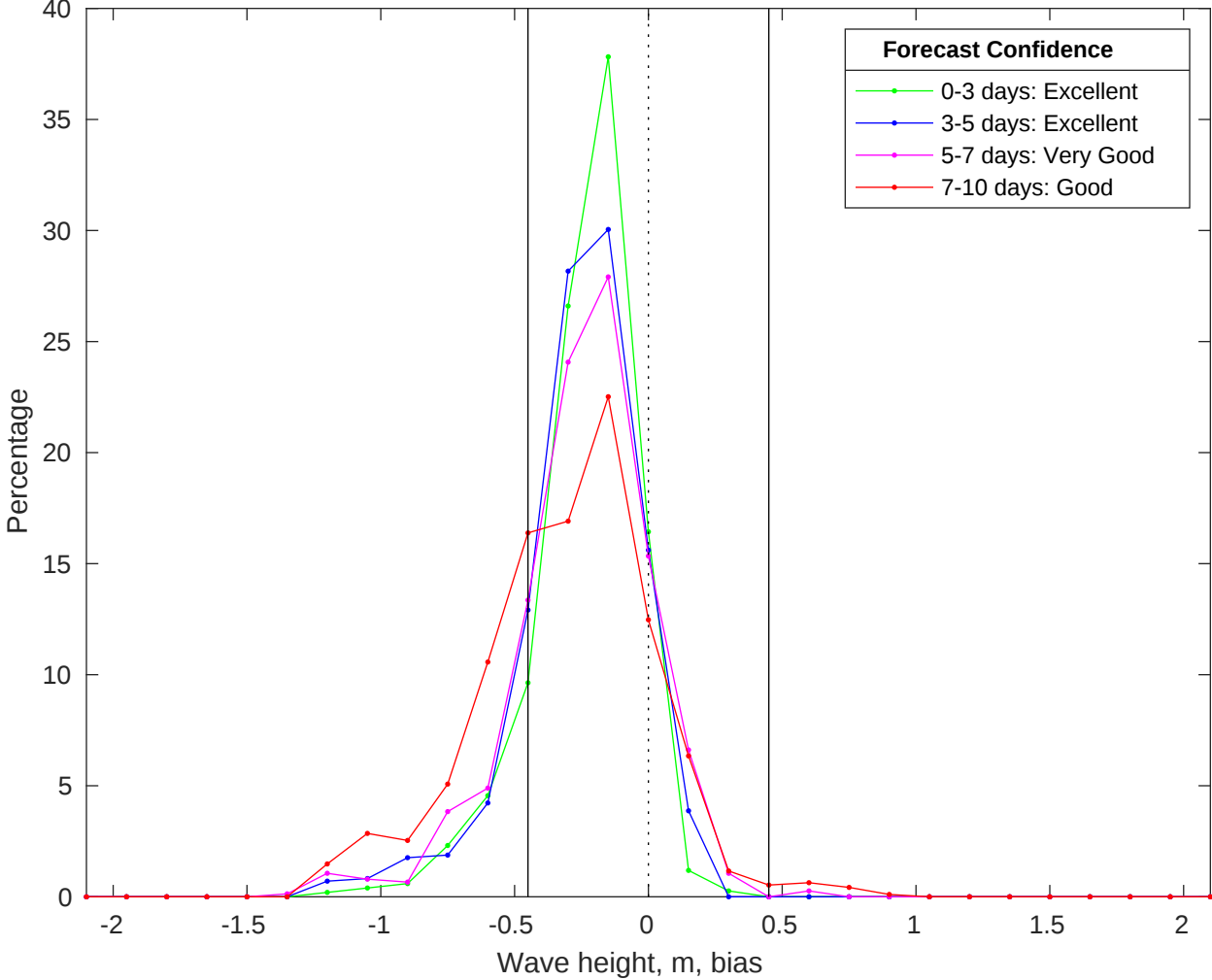
NDBC 42035 vs CMEMS Waves Bias Histogram: 22-May-2025
