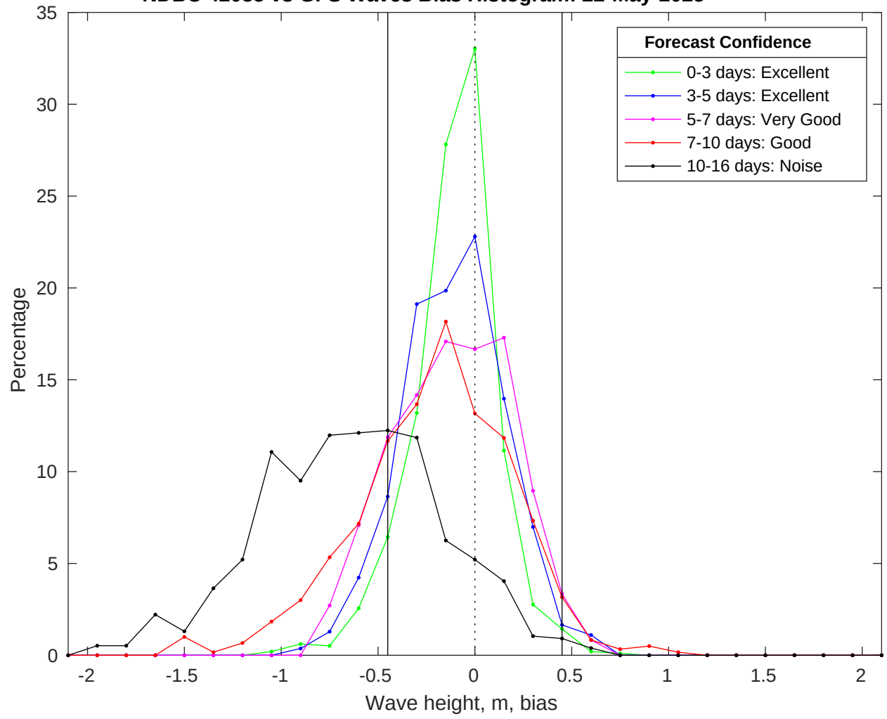
NDBC 42035 vs GFS Waves Bias Histogram: 22-May-2025
