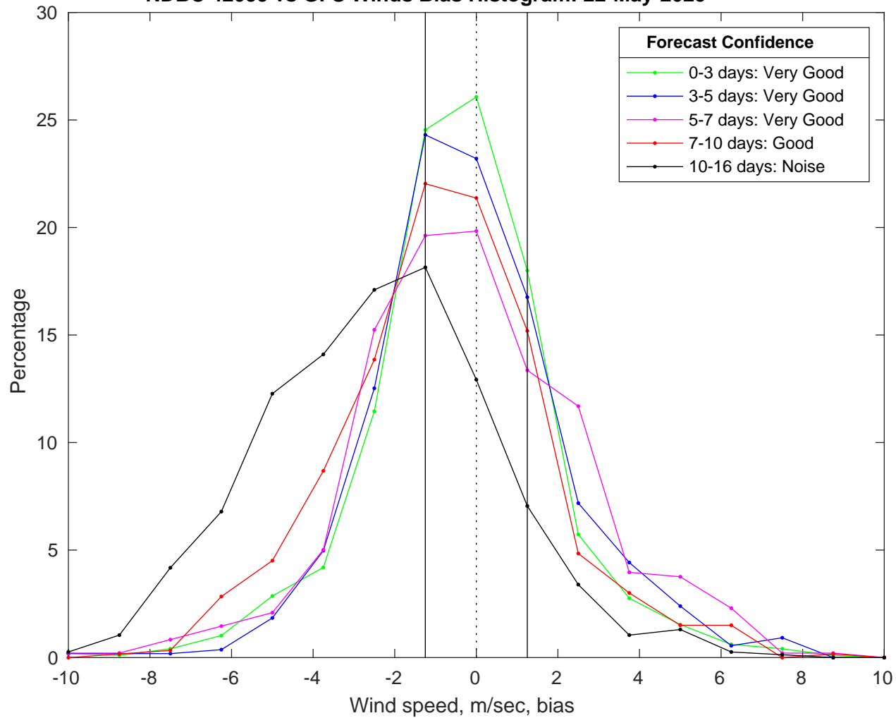
NDBC 42035 vs GFS Winds Bias Histogram: 22-May-2025
