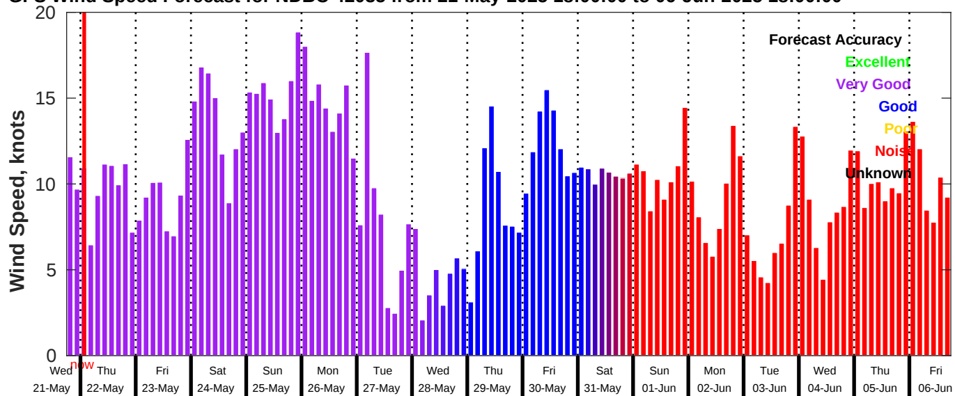
GFS Wind Speed Forecast for NDBC 42035 from 21-May-2025 18:00:00 to 06-Jun-2025 18:00:00
