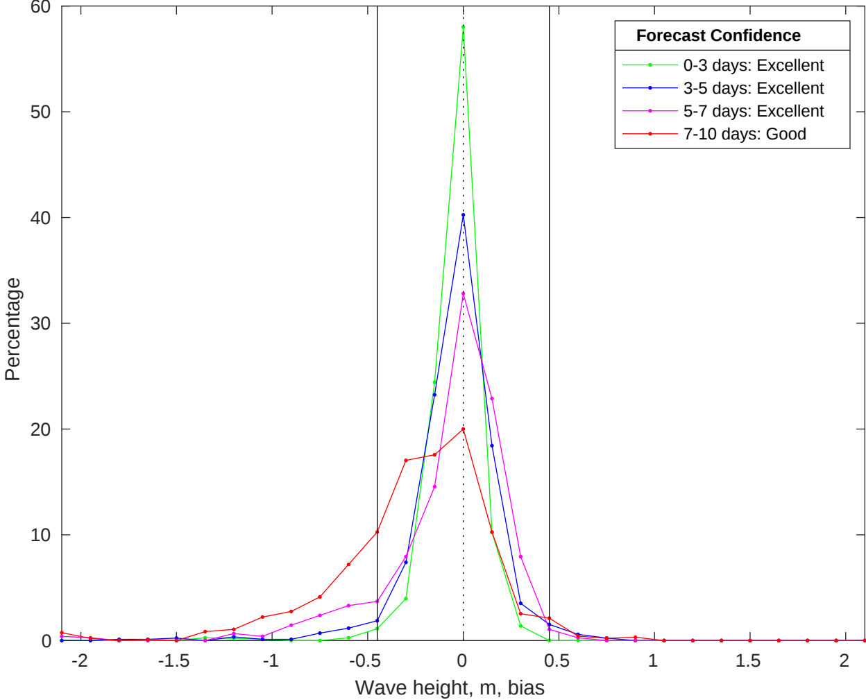
NDBC 42036 vs CMEMS Waves Bias Histogram: 22-May-2025
