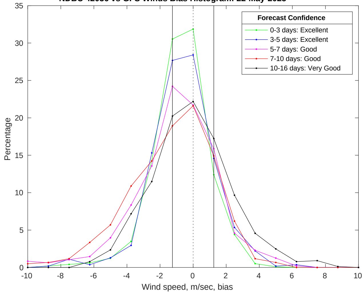
NDBC 42036 vs GFS Winds Bias Histogram: 22-May-2025
