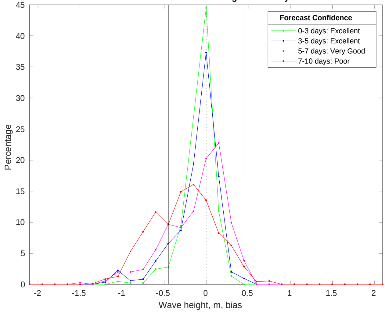
NDBC 42040 vs CMEMS Waves Bias Histogram: 22-May-2025
