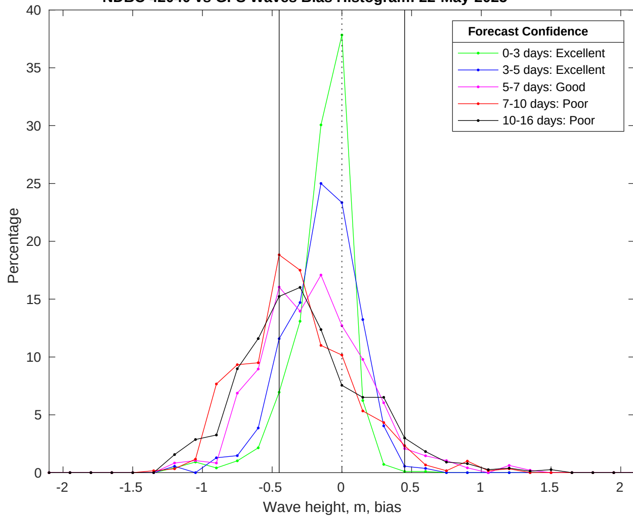
NDBC 42040 vs GFS Waves Bias Histogram: 22-May-2025
